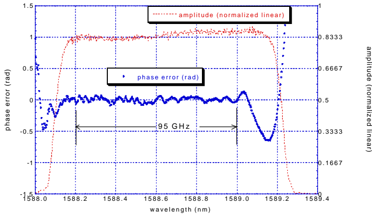
Figure 5. Plot of the phase deviation from parabolic of the data shown in Figure 4. This grating would introduce very little phase (<0.2 radians) distortion over a 95 GHz bandwidth.
