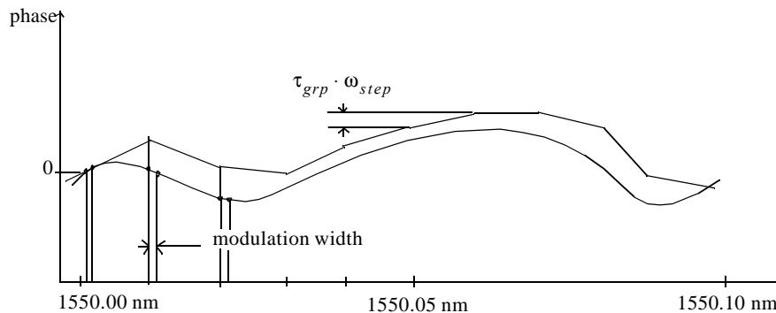
Figure 1. Graphical description of the phase reconstruction process from a typical modulation phase-shift technique (200 MHz modulation, 10 pm step size). Note that in addition to the uncertainty of the group delay measurement, effects of uncertainty in the wavelength at which the measurement was taken must also be taken into account.
