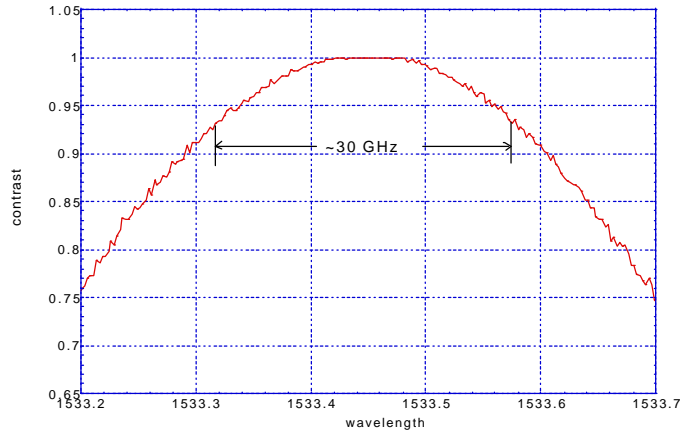
Figure 7. Plot of the effective polarization spectrum of a PM fiber patchcord having a differential group delay of 7 ps. The effective polarization spectrum was computed from the Jones Matrix representing the device using Equation 10.
