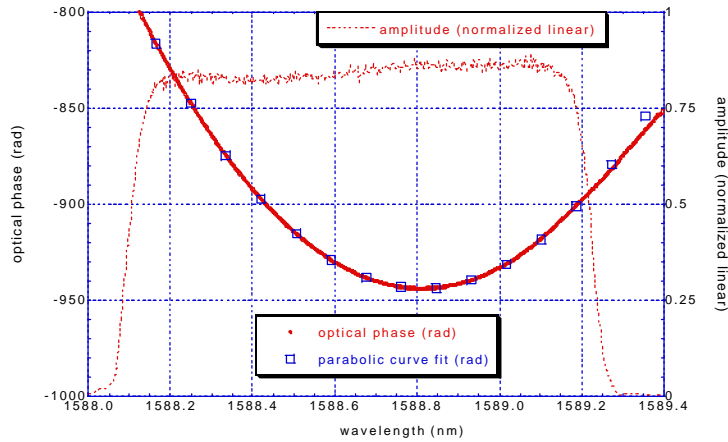
Figure 4. Graph of the amplitude and phase characteristics of a dispersion compensating fiber Bragg grating. Selected points of a parabolic curve fit to the phase data are also shown to illustrate the accuracy of the phase profile.
