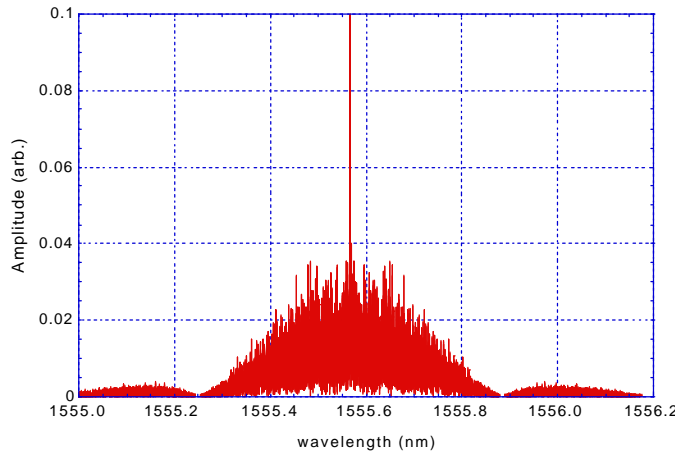
Figure 3. A calculated spectrum of a 40 Gb/s NRZ signal.
